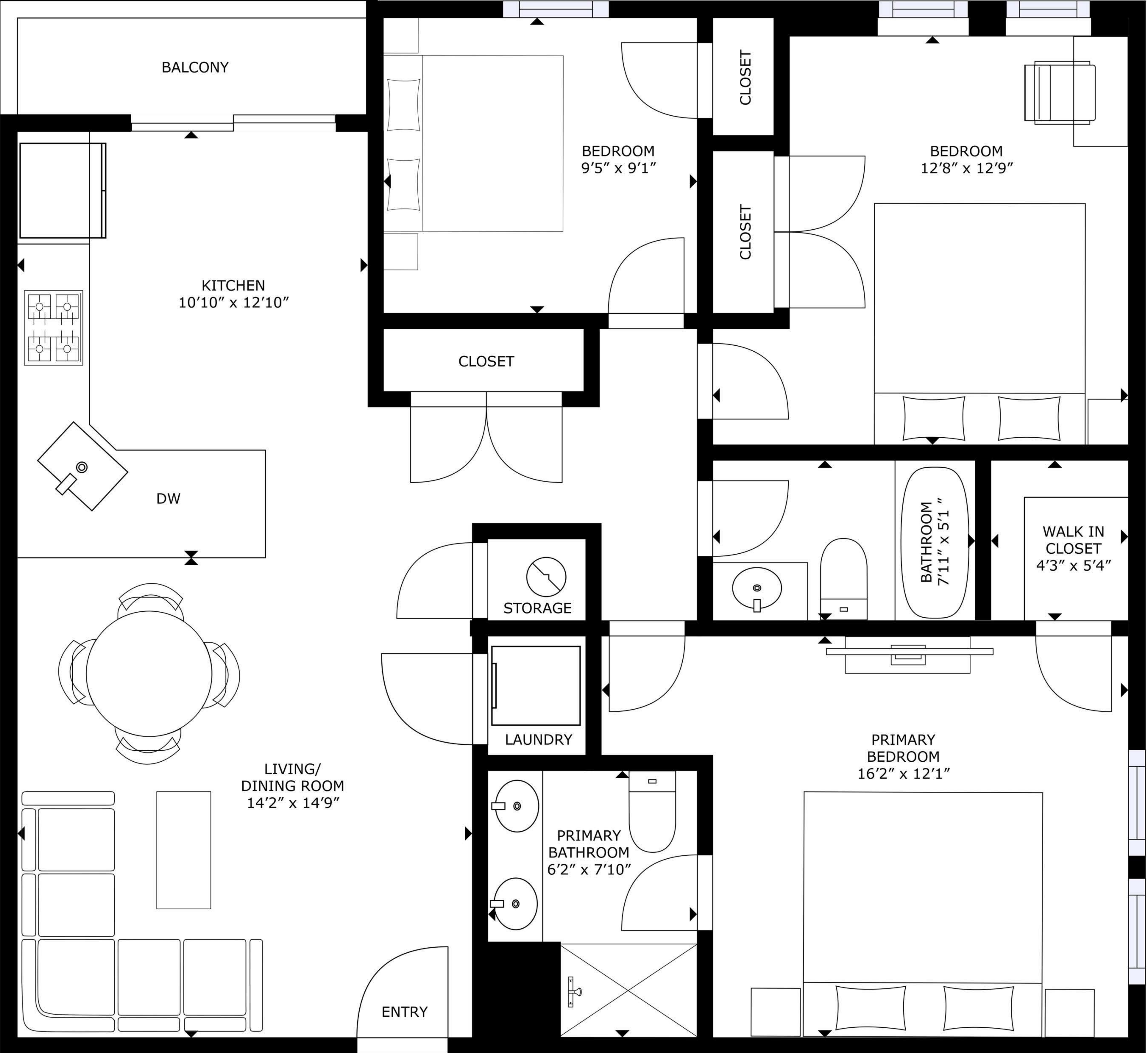
FLOOR PLAN
